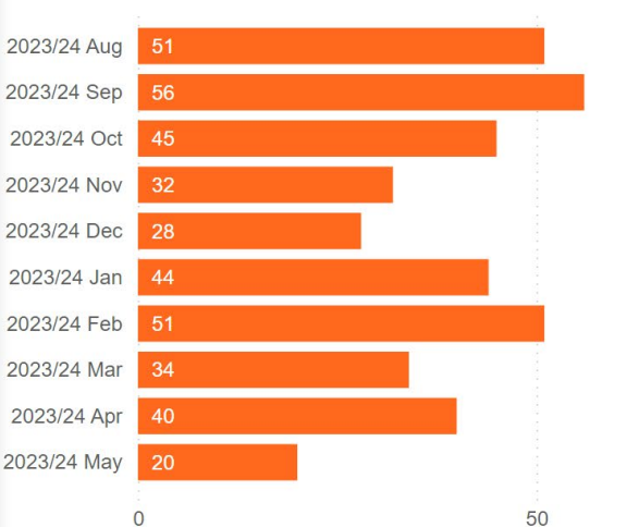
Average Requests
